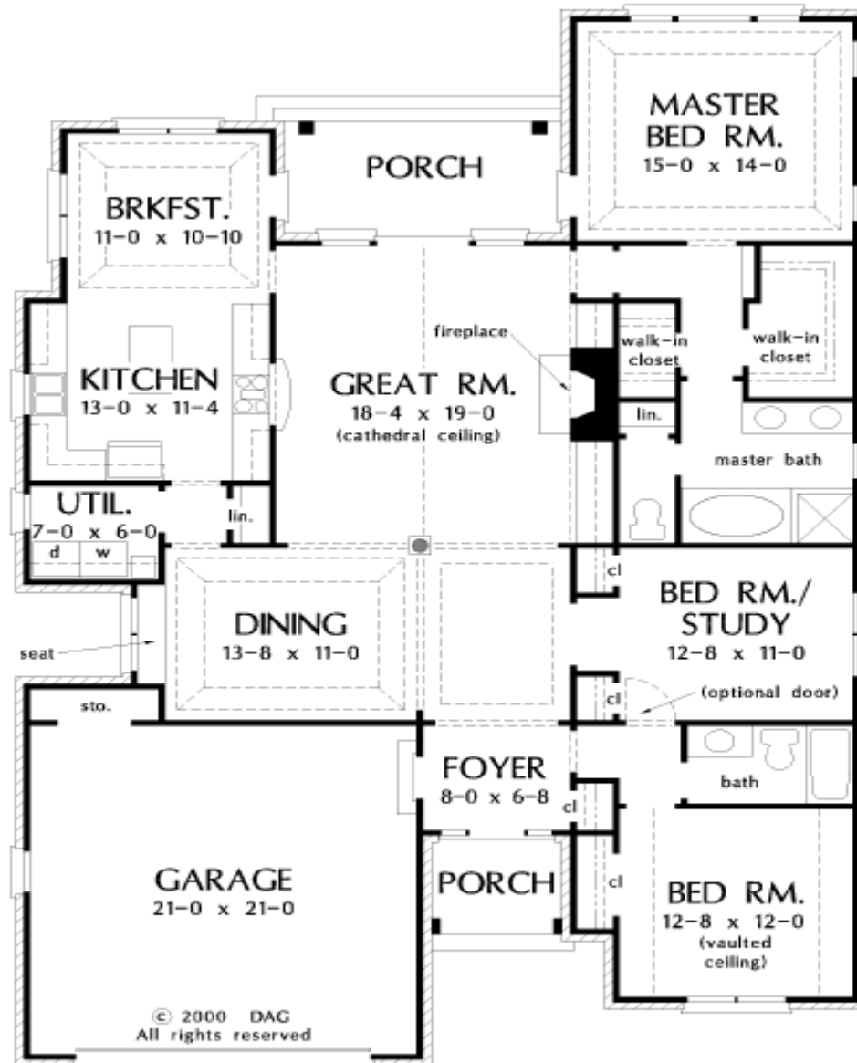
FLOOR PLAN
